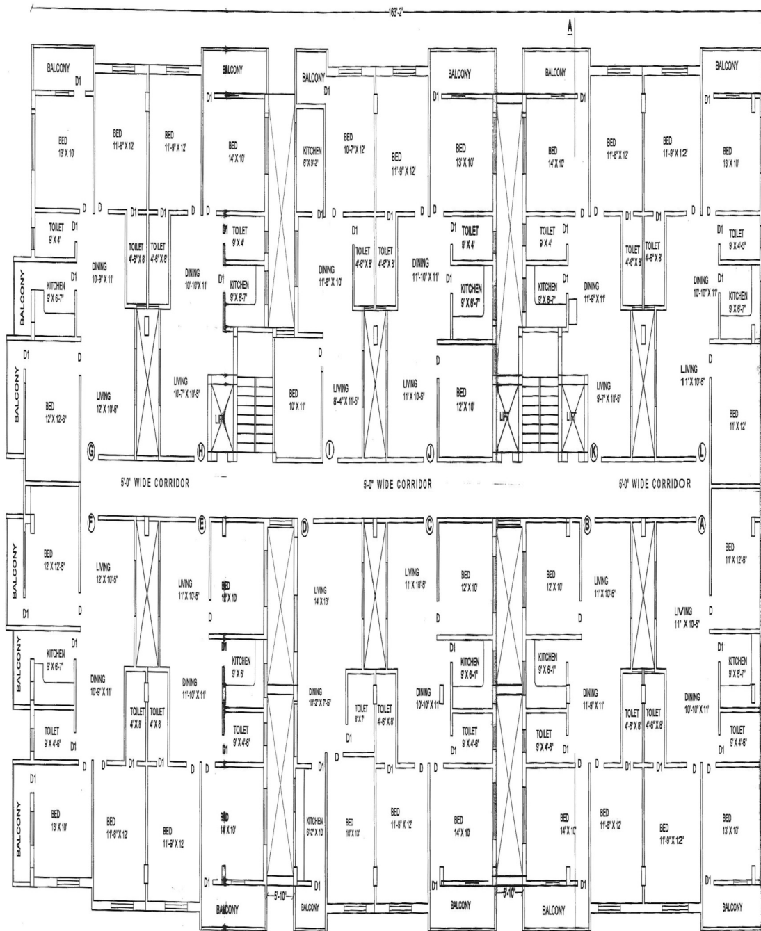
1ST, 2ND, 3RD, & 4TH. FLOOR PLAN
